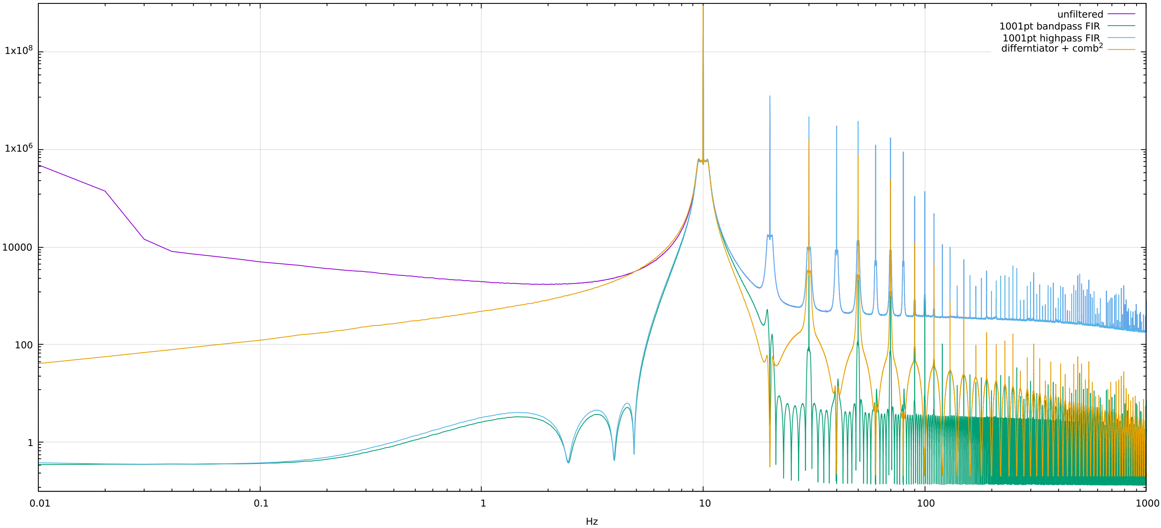
Beat frequency spectrum with PLL enabled
