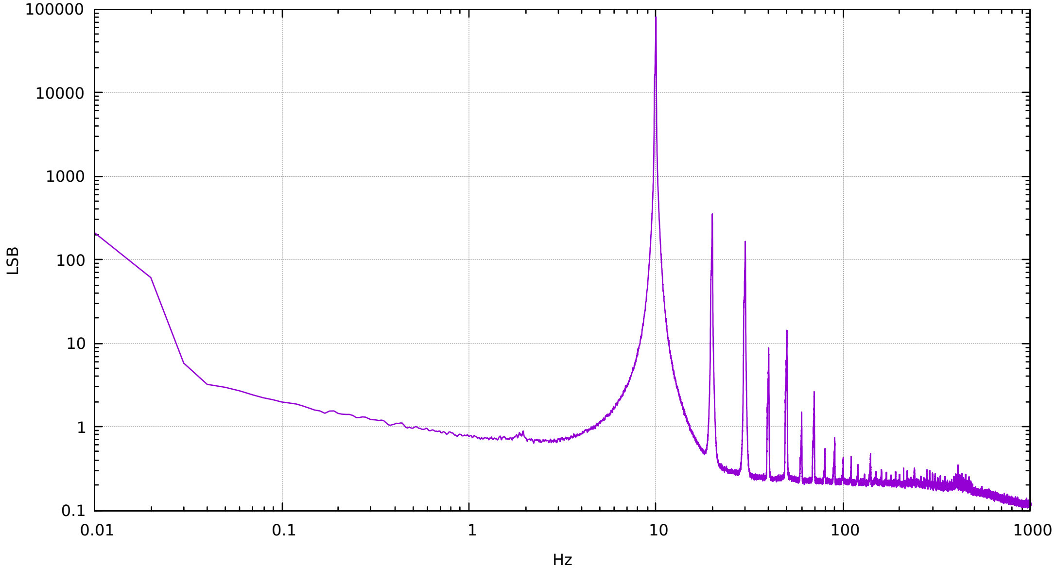
PSD for Abracon AOCJY1 OCXO into the LTC2140 through a resistive divider, after a SINC 2 filter with 1:50 decimation
