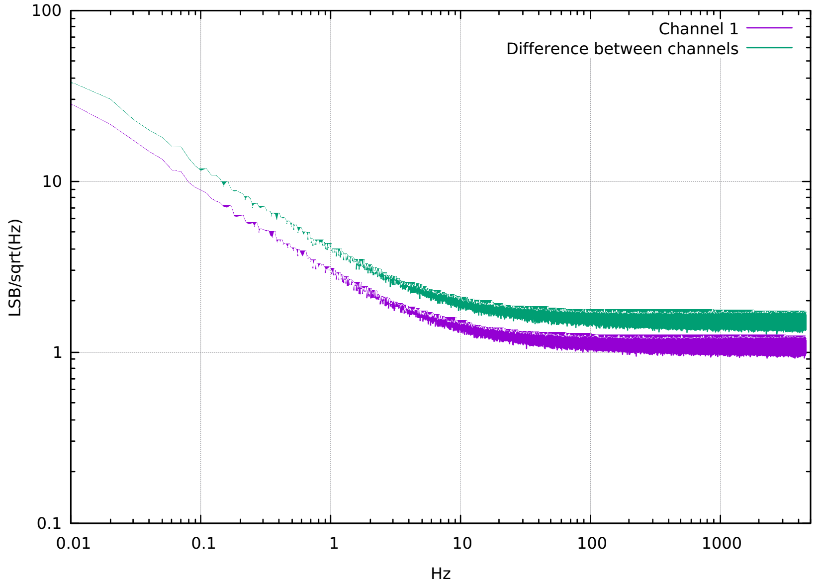
Noise PSD of an LTC2140-14
