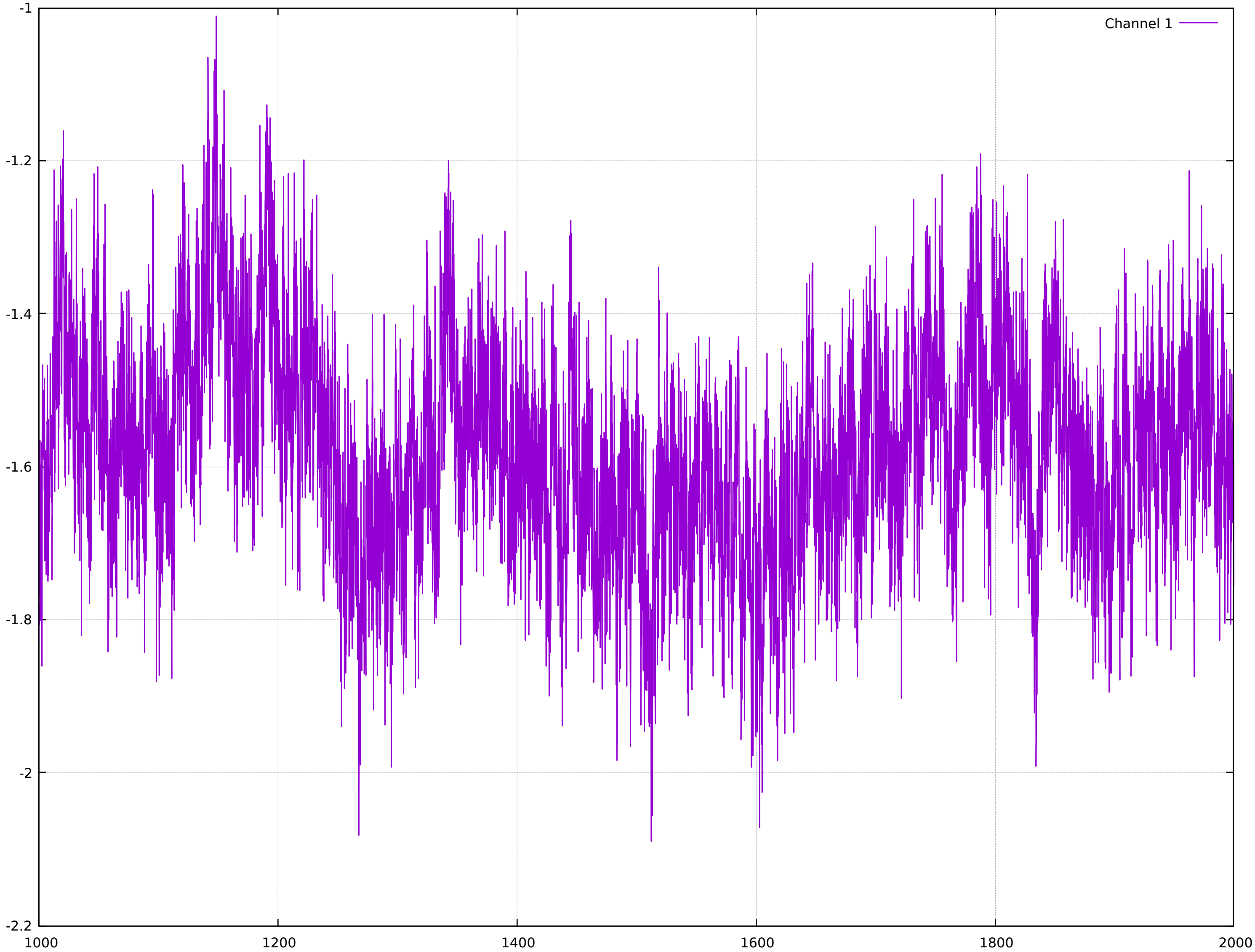
Drift of an LTC2140-14, averaged over 100ms windows
