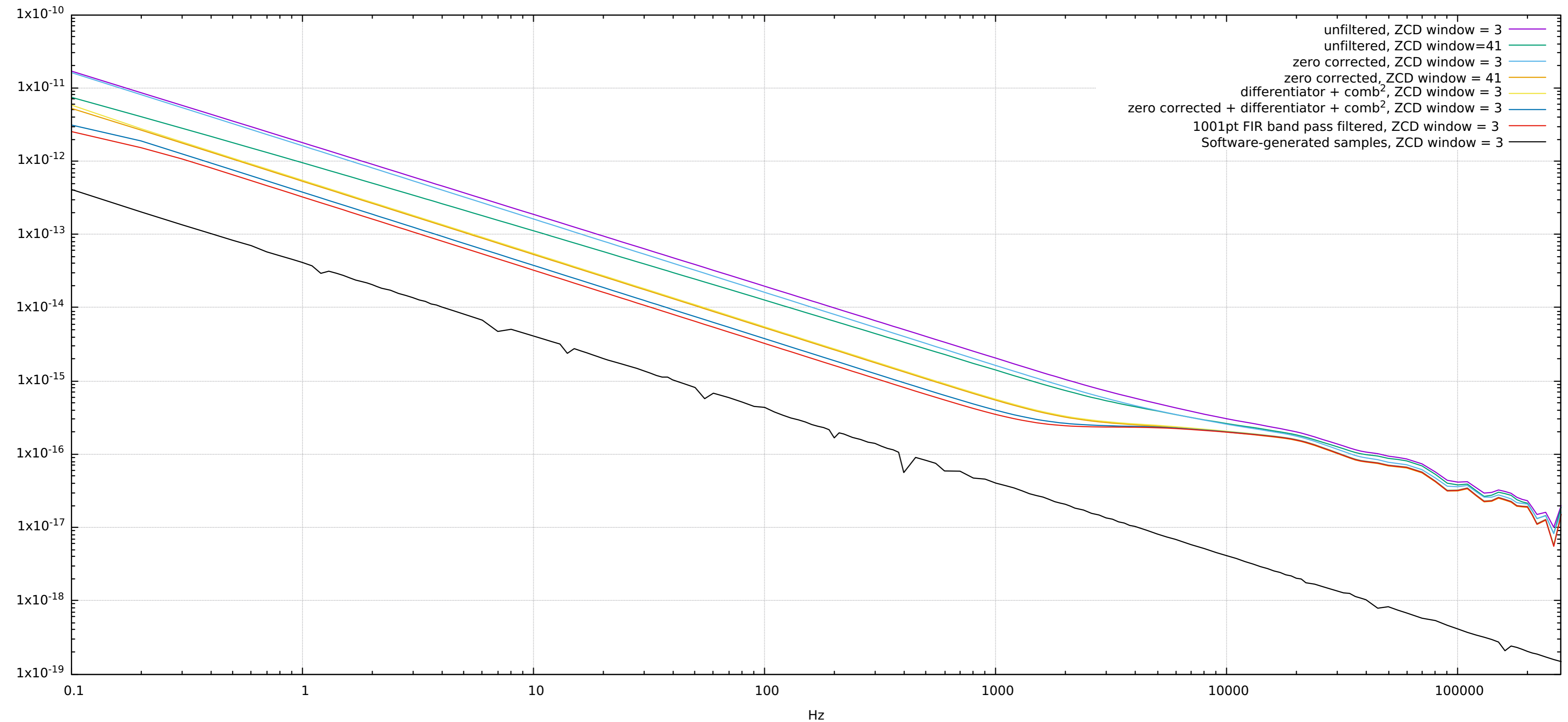
Overlapping ADEV when fed with an 10811 through a splitter
